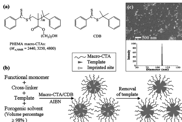
Figure 1. Preparation and characterization of MIP nanoparticles. a) Chemical structures of the RAFT agents used: hydrophilic macro-CTAs and CDB. b) Schematic protocol for the one-pot preparation by RAFTPP of MIP nanoparticles compatible with real aqueous solutions. c) Characterization of MIP nanoparticles ( M_{n,NMR} of PHEMA brushes: 4800) by SEM and DLS.
